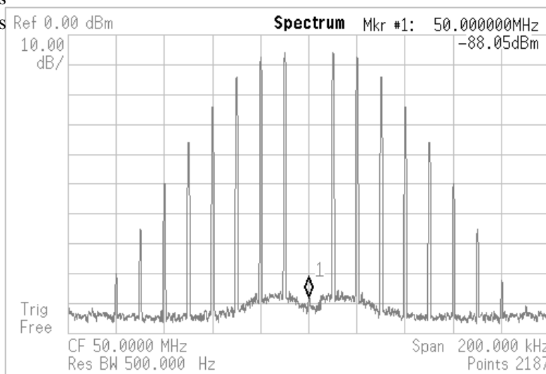
Waveform 6: 50 MHz with FM Carrier Suppressed
